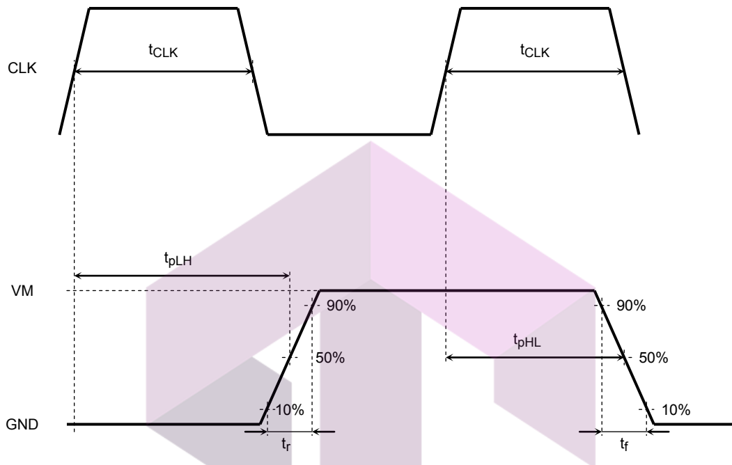
Figure 1 Timing Waveforms and Symbols
